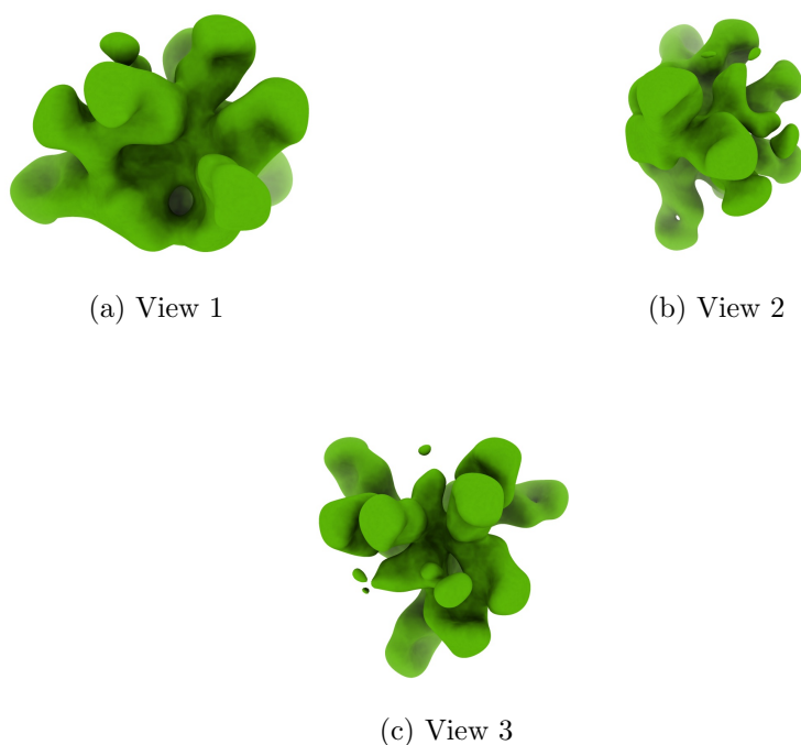
Figure 4: Isosurface at threshold=0.014200. Views generated by ChimeraX at a the following X, Y, Z angles: View 1 (0, -90, -90), View 2 (-90, 0, -90), View 3 (0, 0, 0).
