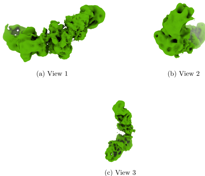
Figure 4: Isosurface at threshold=0.017600. Views generated by ChimeraX at a the following X, Y, Z angles: View 1 (0, -90, -90), View 2 (-90, 0, -90), View 3 (0, 0, 0).
