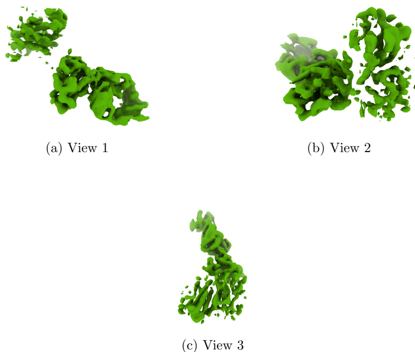
Figure 4: Isosurface at threshold=0.036900. Views generated by ChimeraX at a the following X, Y, Z angles: View 1 (0, -90, -90), View 2 (-90, 0, -90), View 3 (0, 0, 0).
