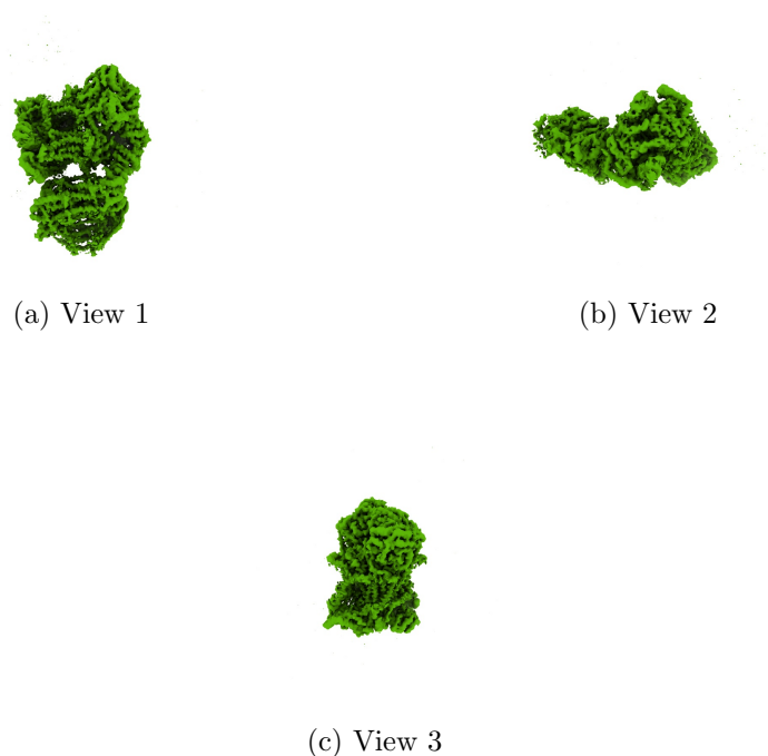
Figure 4: Isosurface at threshold=0.388000. Views generated by ChimeraX at a the following X, Y, Z angles: View 1 (0, -90, -90), View 2 (-90, 0, -90), View 3 (0, 0, 0).
