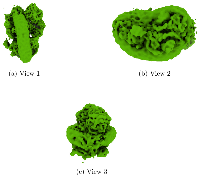
Figure 4: Isosurface at threshold=0.253000. Views generated by ChimeraX at a the following X, Y, Z angles: View 1 (0, -90, -90), View 2 (-90, 0, -90), View 3 (0, 0, 0).
