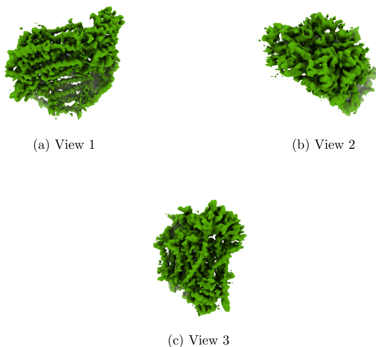
Figure 4: Isosurface at threshold=0.479000. Views generated by ChimeraX at a the following X, Y, Z angles: View 1 (0, -90, -90), View 2 (-90, 0, -90), View 3 (0, 0, 0).
