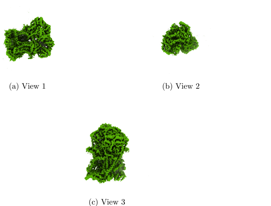
Figure 4: Isosurface at threshold=0.518000. Views generated by ChimeraX at a the following X, Y, Z angles: View 1 (0, -90, -90), View 2 (-90, 0, -90), View 3 (0, 0, 0).
