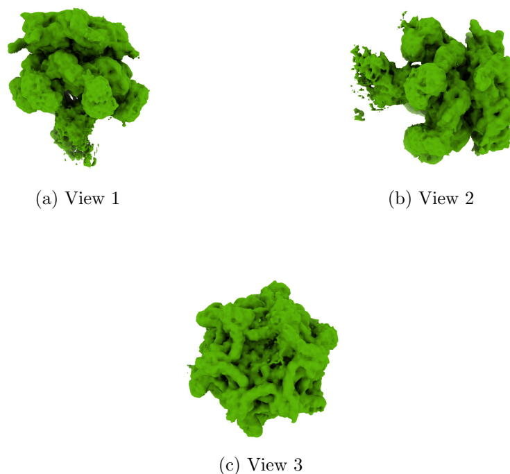
Figure 4: Isosurface at threshold=0.008000. Views generated by ChimeraX at the following X, Y, Z angles: View 1 (0, -90, -90), View 2 (-90, 0, -90), View 3 (0, 0, 0).
