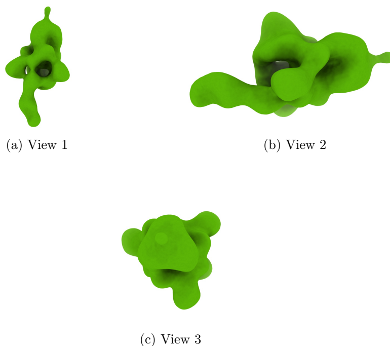
Figure 4: Isosurface at threshold=0.031400. Views generated by ChimeraX at the following X, Y, Z angles: View 1 (0, -90, -90), View 2 (-90, 0, -90), View 3 (0, 0, 0).
