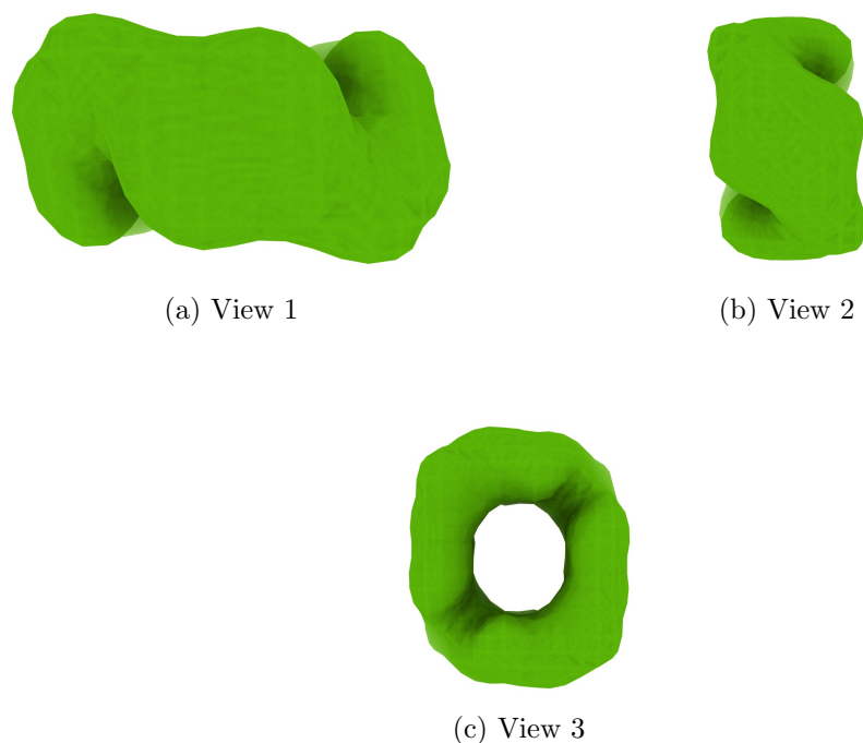
Figure 4: Isosurface at threshold=0.610000. Views generated by ChimeraX at a the following X, Y, Z angles: View 1 (0, -90, -90), View 2 (-90, 0, -90), View 3 (0, 0, 0).
