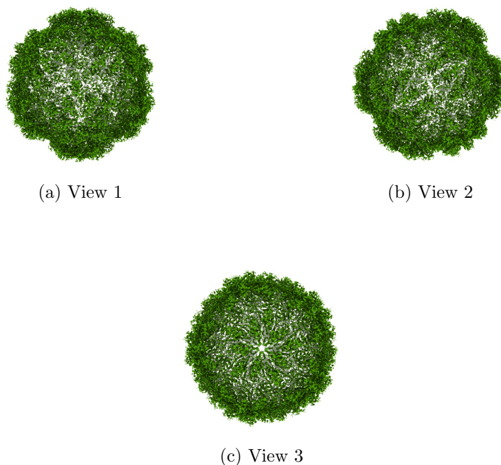
Figure 4: Isosurface at threshold=0.011300. Views generated by ChimeraX at a the following X, Y, Z angles: View 1 (0, -90, -90), View 2 (-90, 0, -90), View 3 (0, 0, 0).
