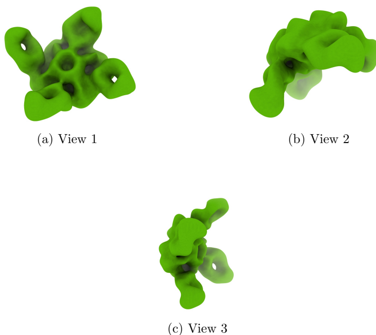
Figure 4: Isosurface at threshold=0.015200. Views generated by ChimeraX at a the following X, Y, Z angles: View 1 (0, -90, -90), View 2 (-90, 0, -90), View 3 (0, 0, 0).
