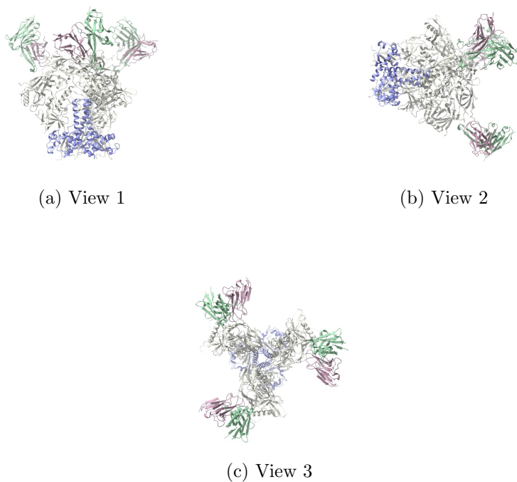
Figure 12: Input atomic model Views generated by ChimeraX at the following X, Y, Z angles: View 1 (0, -90, -90), View 2 (-90, 0, -90), View 3 (0, 0, 0).
