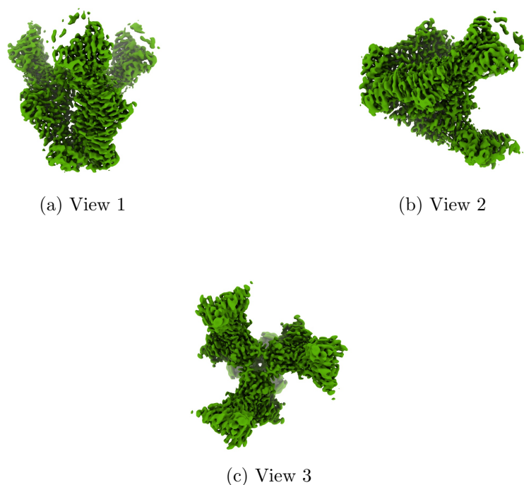
Figure 4: Isosurface at threshold=0.400000. Views generated by ChimeraX at a the following X, Y, Z angles: View 1 (0, -90, -90), View 2 (-90, 0, -90), View 3 (0, 0, 0).
