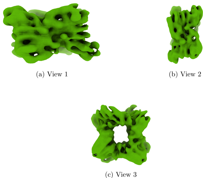
Figure 4: Isosurface at threshold=0.027700. Views generated by ChimeraX at a the following X, Y, Z angles: View 1 (0, -90, -90), View 2 (-90, 0, -90), View 3 (0, 0, 0).
