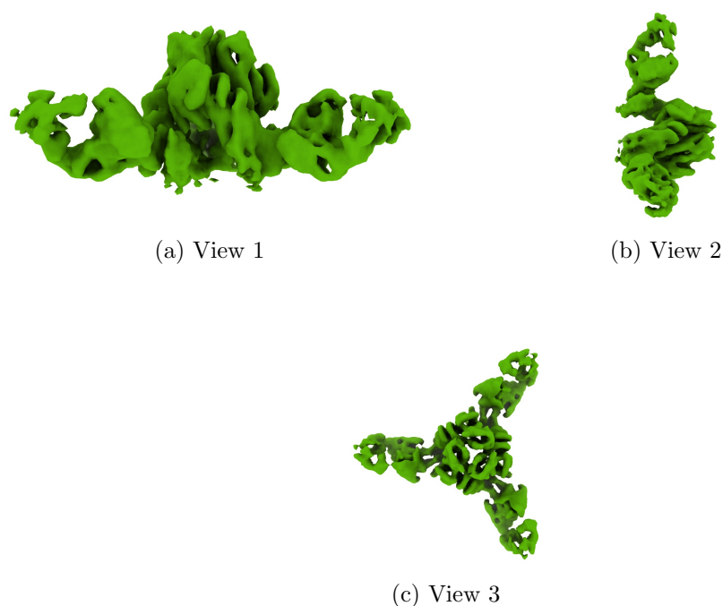
Figure 4: Isosurface at threshold=0.550000. Views generated by ChimeraX at a the following X, Y, Z angles: View 1 (0, -90, -90), View 2 (-90, 0, -90), View 3 (0, 0, 0).
