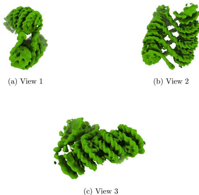
Figure 4: Isosurface at threshold=0.008500. Views generated by ChimeraX at a the following X, Y, Z angles: View 1 (0, -90, -90), View 2 (-90, 0, -90), View 3 (0, 0, 0).
