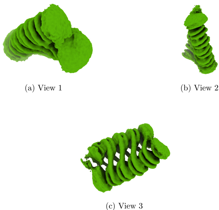
Figure 4: Isosurface at threshold=0.008500. Views generated by ChimeraX at a the following X, Y, Z angles: View 1 (0, -90, -90), View 2 (-90, 0, -90), View 3 (0, 0, 0).
