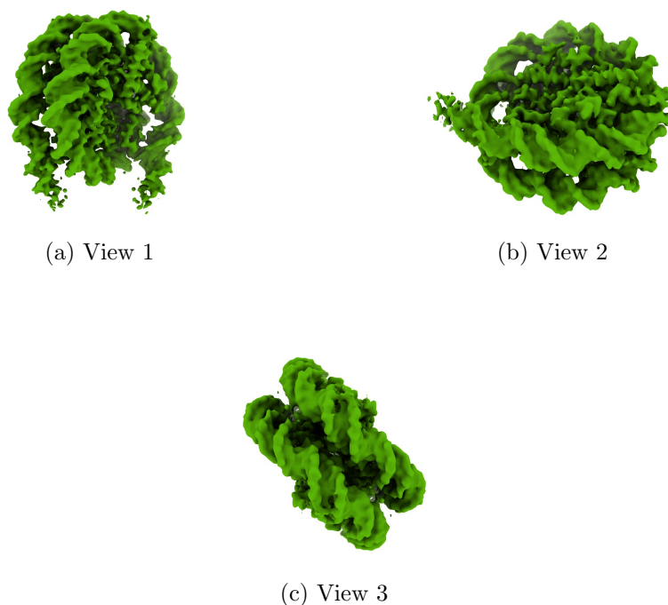
Figure 4: Isosurface at threshold=0.034100. Views generated by ChimeraX at a the following X, Y, Z angles: View 1 (0, -90, -90), View 2 (-90, 0, -90), View 3 (0, 0, 0).
