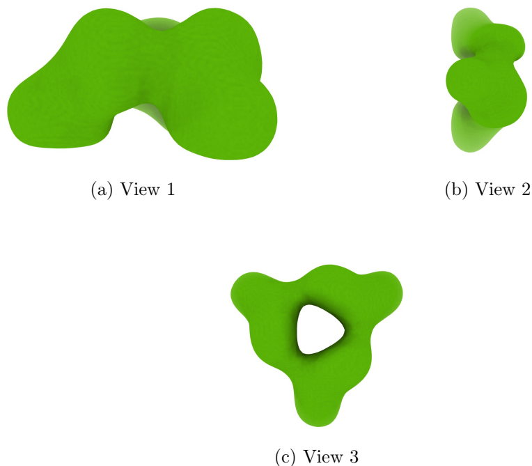
Figure 4: Isosurface at threshold=0.087000. Views generated by ChimeraX at a the following X, Y, Z angles: View 1 (0, -90, -90), View 2 (-90, 0, -90), View 3 (0, 0, 0).
