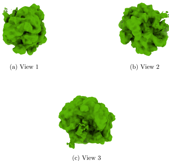
Figure 4: Isosurface at threshold=0.175000. Views generated by ChimeraX at a the following X, Y, Z angles: View 1 (0, -90, -90), View 2 (-90, 0, -90), View 3 (0, 0, 0).
