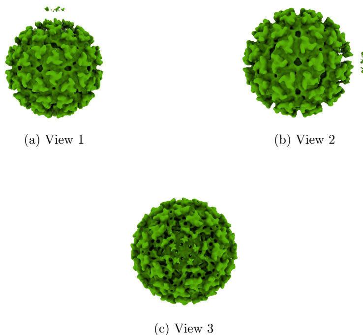
Figure 4: Isosurface at threshold=14.900000. Views generated by ChimeraX at a the following X, Y, Z angles: View 1 (0, -90, -90), View 2 (-90, 0, -90), View 3 (0, 0, 0).
