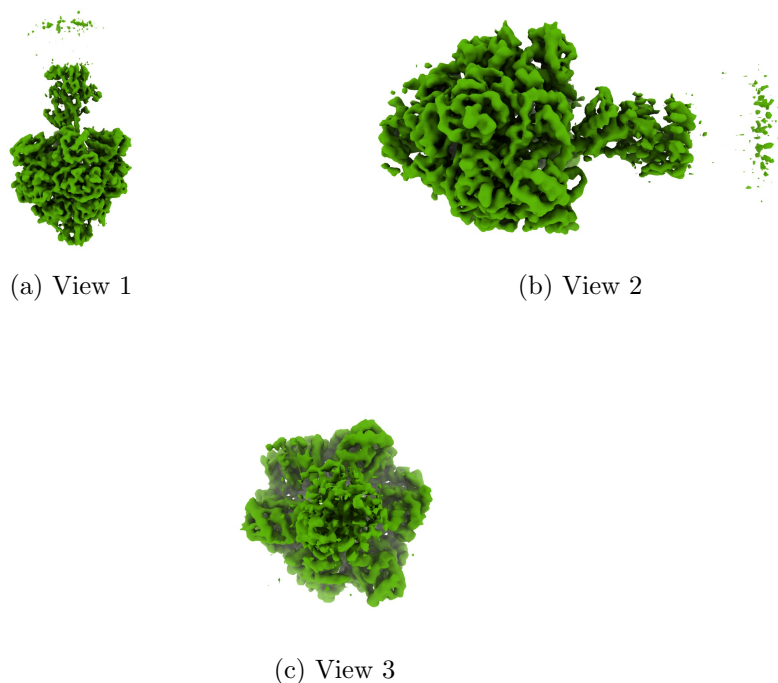
Figure 4: Isosurface at threshold=0.550000. Views generated by ChimeraX at a the following X, Y, Z angles: View 1 (0, -90, -90), View 2 (-90, 0, -90), View 3 (0, 0, 0).
