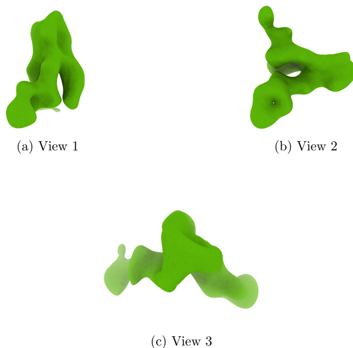
Figure 4: Isosurface at threshold=0.022700. Views generated by ChimeraX at a the following X, Y, Z angles: View 1 (0, -90, -90), View 2 (-90, 0, -90), View 3 (0, 0, 0).
