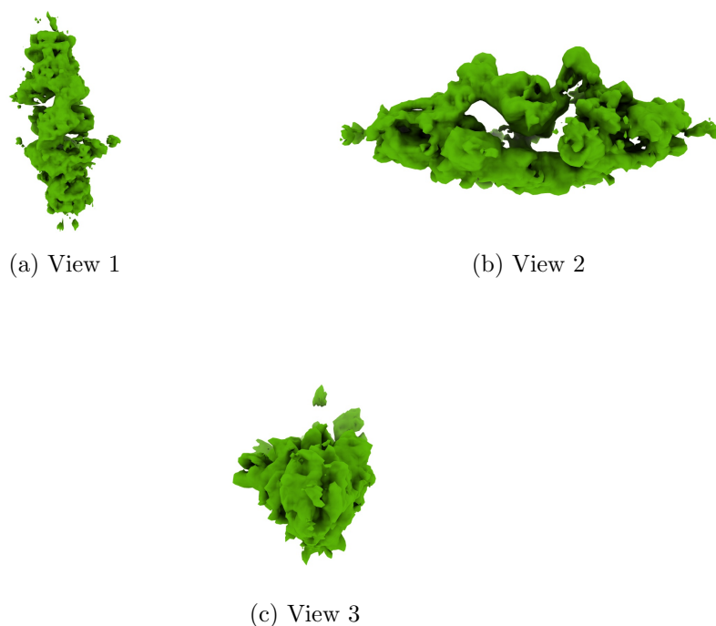
Figure 4: Isosurface at threshold=0.350000. Views generated by ChimeraX at a the following X, Y, Z angles: View 1 (0, -90, -90), View 2 (-90, 0, -90), View 3 (0, 0, 0).
