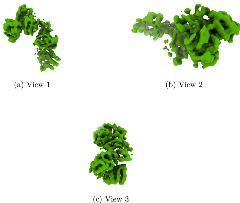
Figure 4: Isosurface at threshold=0.003700. Views generated by ChimeraX at a the following X, Y, Z angles: View 1 (0, -90, -90), View 2 (-90, 0, -90), View 3 (0, 0, 0).
