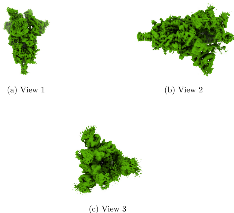
Figure 4: Isosurface at threshold=0.149000. Views generated by ChimeraX at a the following X, Y, Z angles: View 1 (0, -90, -90), View 2 (-90, 0, -90), View 3 (0, 0, 0).
