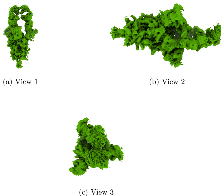
Figure 4: Isosurface at threshold=0.143000. Views generated by ChimeraX at a the following X, Y, Z angles: View 1 (0, -90, -90), View 2 (-90, 0, -90), View 3 (0, 0, 0).
