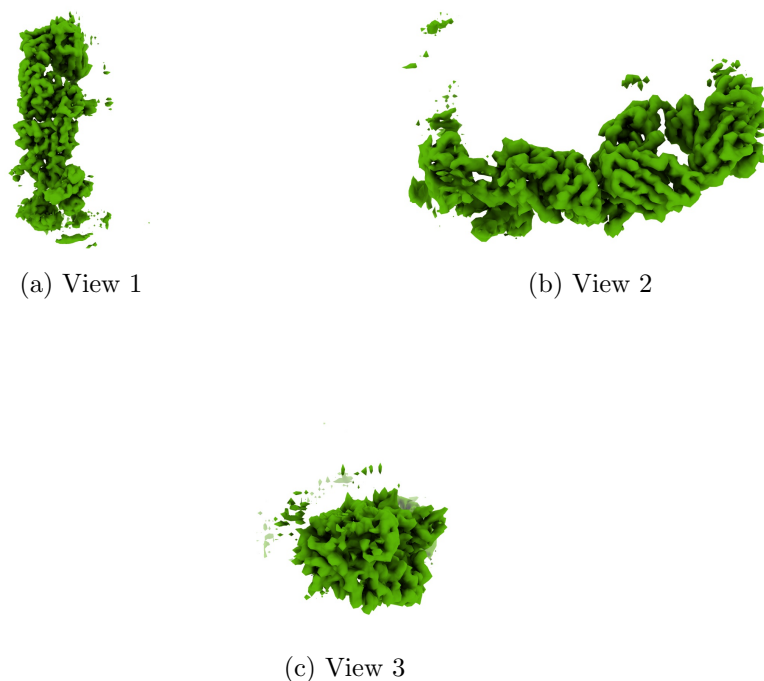
Figure 4: Isosurface at threshold=0.238000. Views generated by ChimeraX at a the following X, Y, Z angles: View 1 (0, -90, -90), View 2 (-90, 0, -90), View 3 (0, 0, 0).
