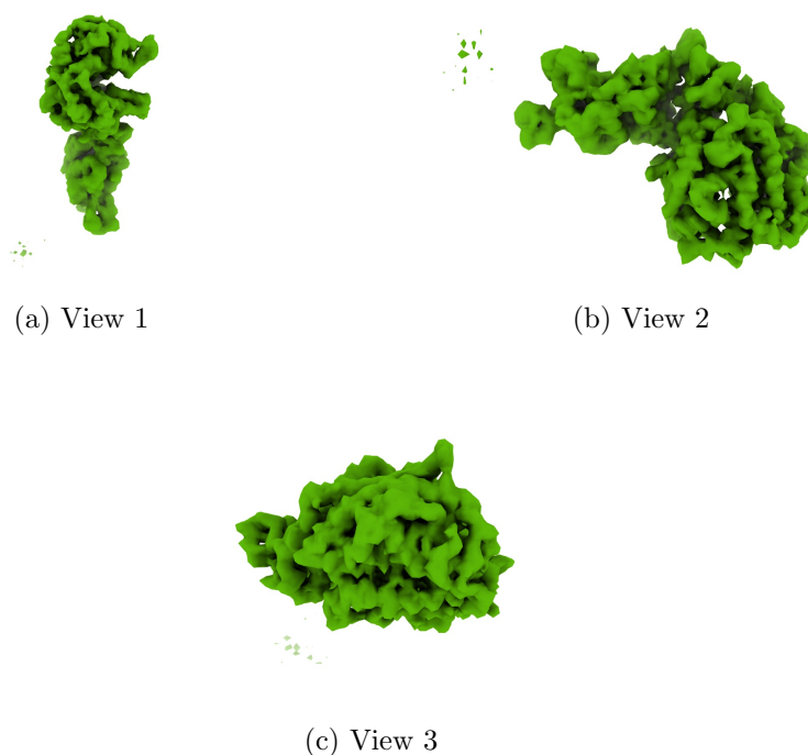
Figure 4: Isosurface at threshold=0.192000. Views generated by ChimeraX at a the following X, Y, Z angles: View 1 (0, -90, -90), View 2 (-90, 0, -90), View 3 (0, 0, 0).
