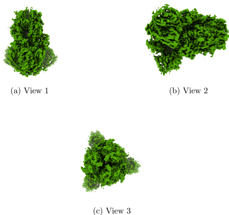
Figure 4: Isosurface at threshold=0.089000. Views generated by ChimeraX at a the following X, Y, Z angles: View 1 (0, -90, -90), View 2 (-90, 0, -90), View 3 (0, 0, 0).
