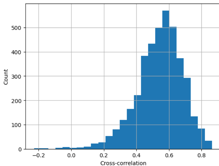
Figure 19: Histogram of the cross-correlation between the map and model evaluated for all residues.
