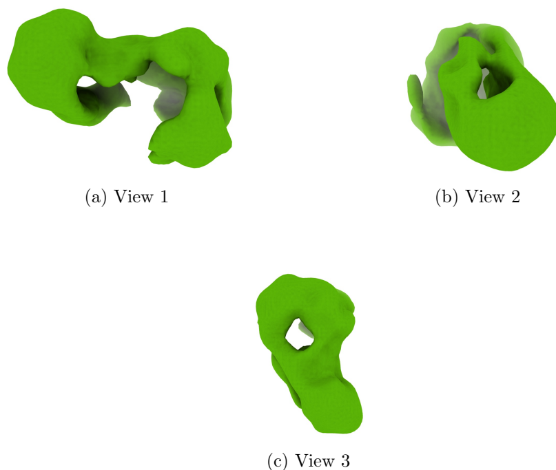
Figure 4: Isosurface at threshold=0.093800. Views generated by ChimeraX at a the following X, Y, Z angles: View 1 (0, -90, -90), View 2 (-90, 0, -90), View 3 (0, 0, 0).
