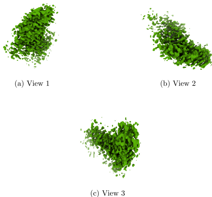
Figure 4: Isosurface at threshold=0.006900. Views generated by ChimeraX at a the following X, Y, Z angles: View 1 (0, -90, -90), View 2 (-90, 0, -90), View 3 (0, 0, 0).
