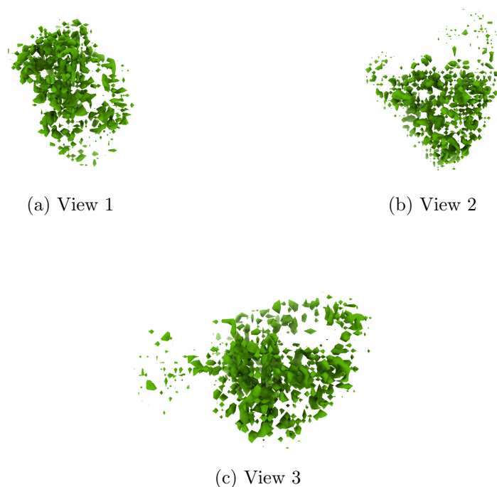
Figure 4: Isosurface at threshold=0.028300. Views generated by ChimeraX at a the following X, Y, Z angles: View 1 (0, -90, -90), View 2 (-90, 0, -90), View 3 (0, 0, 0).
