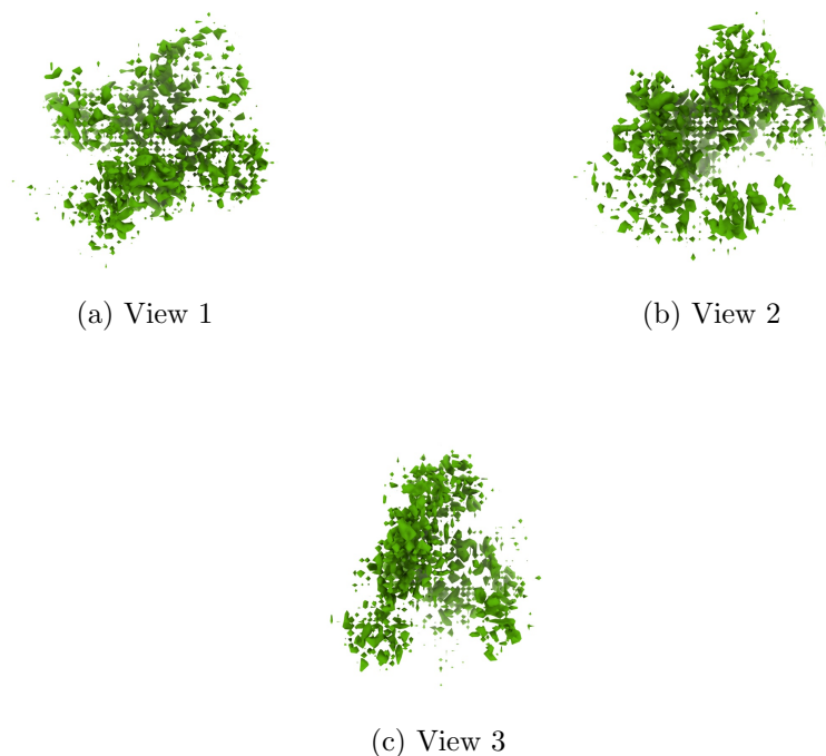
Figure 4: Isosurface at threshold=0.027100. Views generated by ChimeraX at a the following X, Y, Z angles: View 1 (0, -90, -90), View 2 (-90, 0, -90), View 3 (0, 0, 0).
