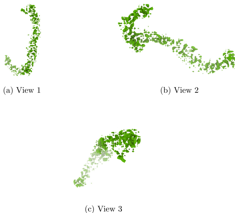
Figure 4: Isosurface at threshold=0.030100. Views generated by ChimeraX at a the following X, Y, Z angles: View 1 (0, -90, -90), View 2 (-90, 0, -90), View 3 (0, 0, 0).
