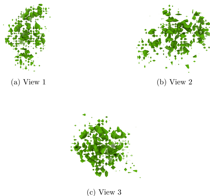
Figure 4: Isosurface at threshold=0.030600. Views generated by ChimeraX at a the following X, Y, Z angles: View 1 (0, -90, -90), View 2 (-90, 0, -90), View 3 (0, 0, 0).
