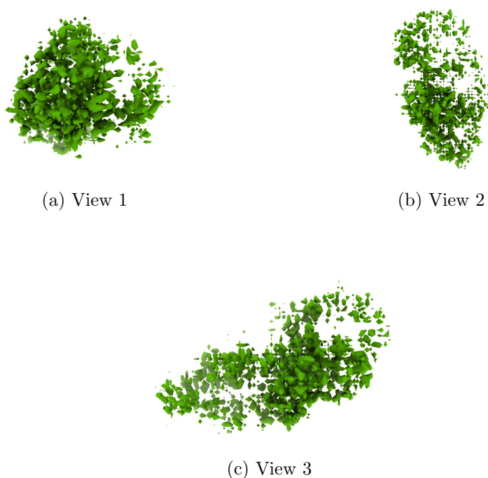
Figure 4: Isosurface at threshold=0.032800. Views generated by ChimeraX at a the following X, Y, Z angles: View 1 (0, -90, -90), View 2 (-90, 0, -90), View 3 (0, 0, 0).
