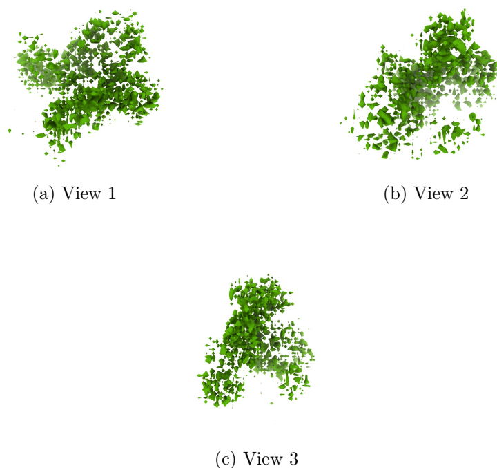
Figure 4: Isosurface at threshold=0.031500. Views generated by ChimeraX at a the following X, Y, Z angles: View 1 (0, -90, -90), View 2 (-90, 0, -90), View 3 (0, 0, 0).
