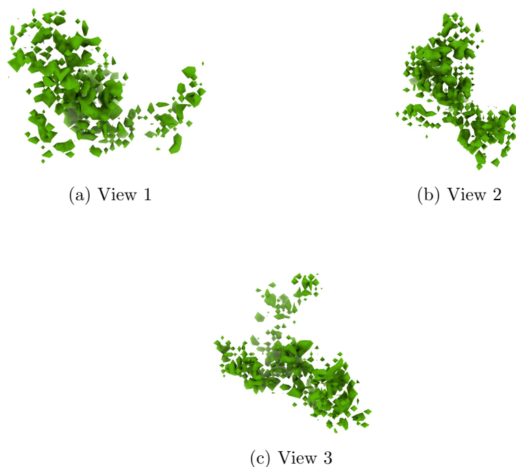
Figure 4: Isosurface at threshold=0.033800. Views generated by ChimeraX at a the following X, Y, Z angles: View 1 (0, -90, -90), View 2 (-90, 0, -90), View 3 (0, 0, 0).
