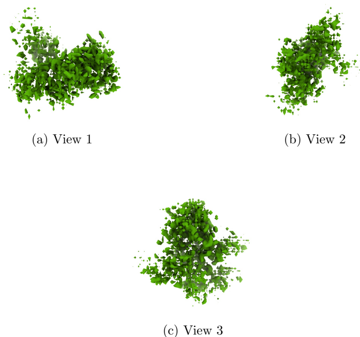
Figure 4: Isosurface at threshold=0.031700. Views generated by ChimeraX at a the following X, Y, Z angles: View 1 (0, -90, -90), View 2 (-90, 0, -90), View 3 (0, 0, 0).
