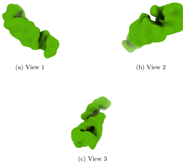
Figure 4: Isosurface at threshold=3.220000. Views generated by ChimeraX at a the following X, Y, Z angles: View 1 (0, -90, -90), View 2 (-90, 0, -90), View 3 (0, 0, 0).
