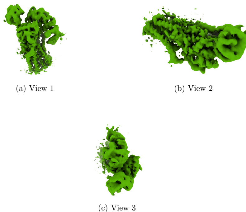
Figure 4: Isosurface at threshold=0.115000. Views generated by ChimeraX at a the following X, Y, Z angles: View 1 (0, -90, -90), View 2 (-90, 0, -90), View 3 (0, 0, 0).
