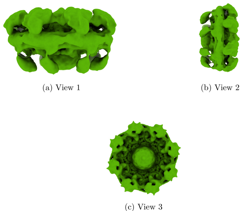
Figure 4: Isosurface at threshold=0.025000. Views generated by ChimeraX at the following X, Y, Z angles: View 1 (0, -90, -90), View 2 (-90, 0, -90), View 3 (0, 0, 0).
