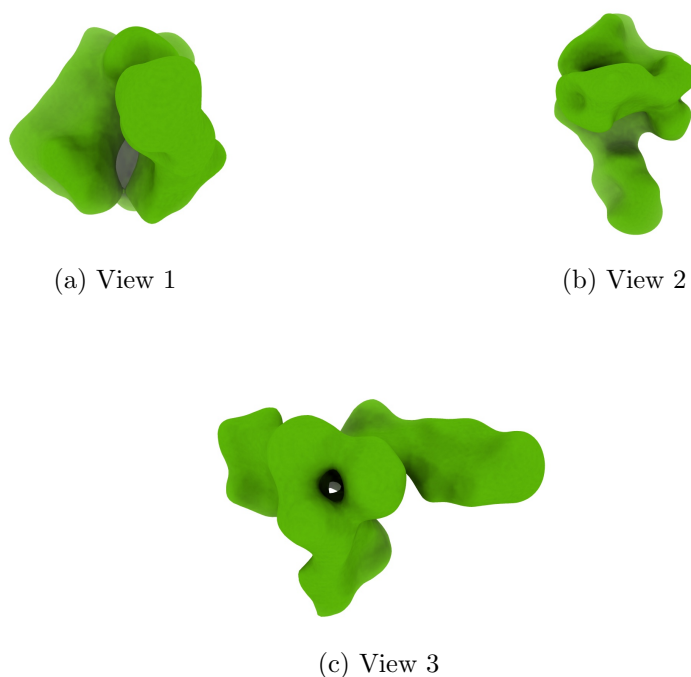
Figure 4: Isosurface at threshold=0.014500. Views generated by ChimeraX at a the following X, Y, Z angles: View 1 (0, -90, -90), View 2 (-90, 0, -90), View 3 (0, 0, 0).
