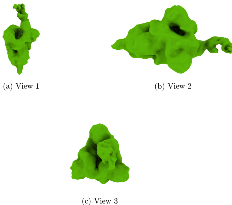
Figure 4: Isosurface at threshold=0.450000. Views generated by ChimeraX at a the following X, Y, Z angles: View 1 (0, -90, -90), View 2 (-90, 0, -90), View 3 (0, 0, 0).
