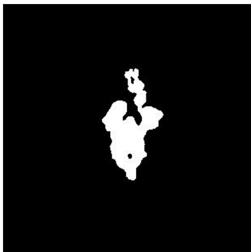
(a) X Slice 153
