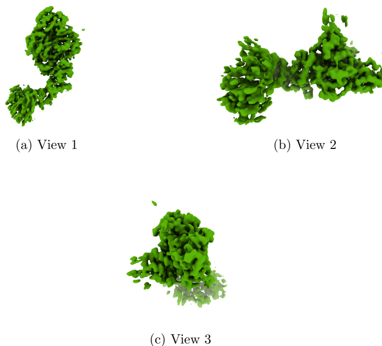
Figure 4: Isosurface at threshold=0.086000. Views generated by ChimeraX at a the following X, Y, Z angles: View 1 (0, -90, -90), View 2 (-90, 0, -90), View 3 (0, 0, 0).
