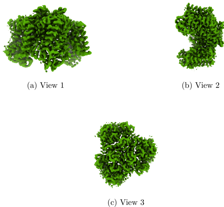
Figure 4: Isosurface at threshold=2.830000. Views generated by ChimeraX at a the following X, Y, Z angles: View 1 (0, -90, -90), View 2 (-90, 0, -90), View 3 (0, 0, 0).
