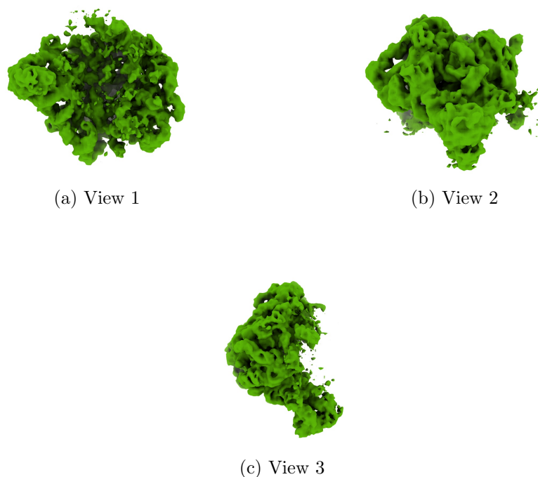
Figure 4: Isosurface at threshold=5.200000. Views generated by ChimeraX at a the following X, Y, Z angles: View 1 (0, -90, -90), View 2 (-90, 0, -90), View 3 (0, 0, 0).
