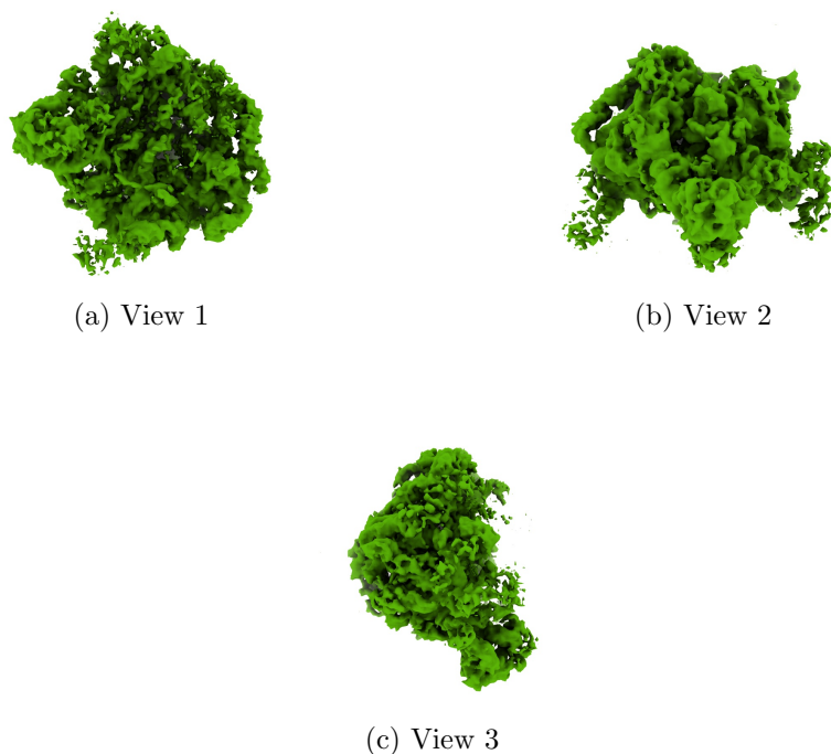
Figure 4: Isosurface at threshold=6.500000. Views generated by ChimeraX at a the following X, Y, Z angles: View 1 (0, -90, -90), View 2 (-90, 0, -90), View 3 (0, 0, 0).
